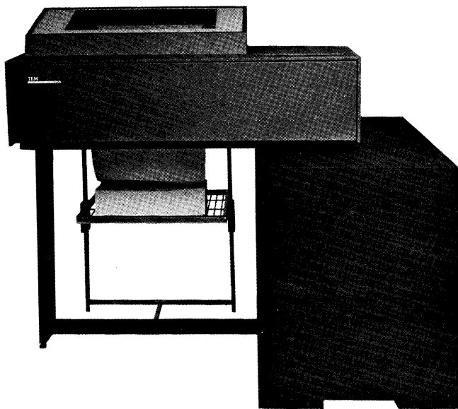
Figure 4. 1443 Printer
