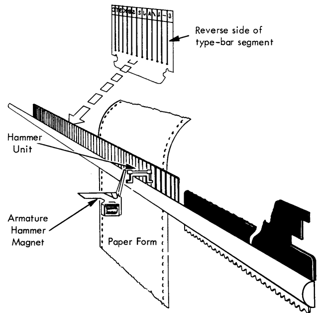
Figure 5. Printing Schematic
