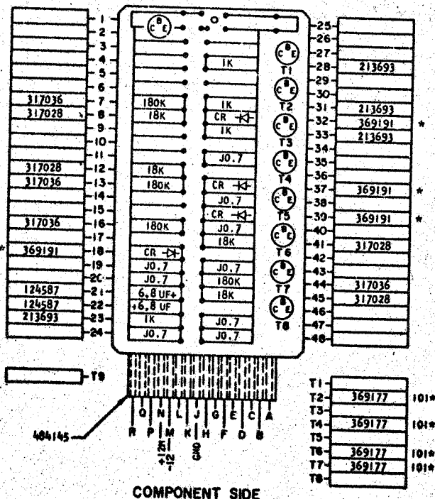
COMPONENT SIDE
